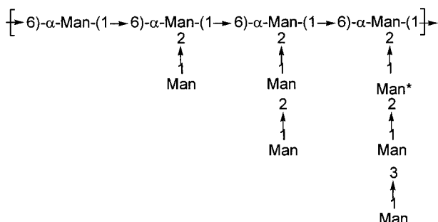
Figure 1. Schematic representation for the polysaccharide structure of the mannan from S. cerevisiae . [19b] The sequential arrangement of the different side chains is arbitrary. The asterisk * indicates the presence of the following substituents at O-6: 30% H, 20% \text{PO}_3^{2-} , 20% \alpha -Man- \text{OPO}_2^{2-} , and 30% \alpha -Man-(1 \rightarrow 3)- \alpha -Man- \text{OPO}_2^{2-} .
