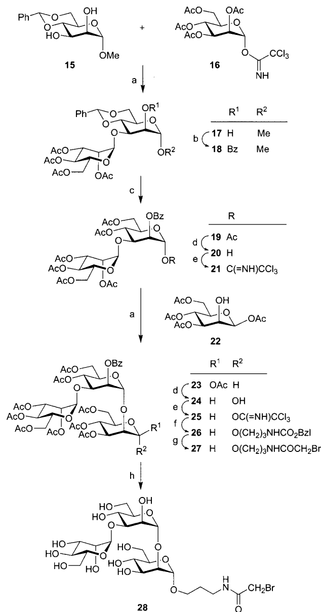
Scheme 3. Synthesis of spacer-armed mannotriptide derivative 28 . a) BF_3 \cdot OEt_2 , CH_2Cl_2 , 83% for 17 , 55% for 23 ; b) BzCl , C_5H_5N , CH_2Cl_2 , 88% over two steps (a and b); c) 1% H_2SO_4 , Ac_2O/AcOH , 78%; d) NH_2NH_2 \cdot HOAc , DMF, 93% for 20 , 85% for 24 ; e) Cl_3CCN , DBU, CH_2Cl_2 , 79% for 21 , 89% for 25 ; f) 2 , TMSOTf, CH_2Cl_2 , 91%; g) 1. H_2 -Pd/C, EtOH/EtOAc ; 2. BrCH_2COBr , CH_2Cl_2 , Et_3N , -50^\circ C , 75%; h) 0.01 M NaOMe, MeOH, 87%.
