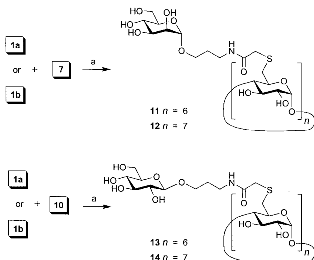
Scheme 2. a) DMF/H 2 O, 2:1, K 2 CO 3 , 64% for 11 , 69% for 12 , 57% for 13 and 75% for 14 .
