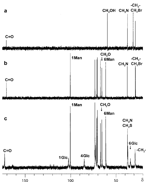
Figure 4. 13 C NMR spectra of 2-bromo-N-(3-hydroxypropyl)acetamide ( 3 ) (a), mannopyranoside 7 (b), and cluster mannopyranoside 12 (c) in D 2 O.
