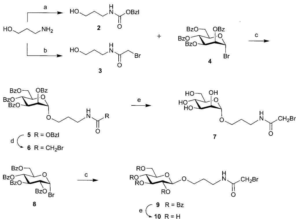
Scheme 1. Synthesis of spacer-armed glycoside derivatives 7 and 10 . a) \text{BzO-CO-Cl} , \text{Na}_2\text{CO}_3 , \text{H}_2\text{O} , 90%; b) 1. \text{BrCH}_2\text{COBr} , \text{CH}_2\text{Cl}_2 , \text{Et}_3\text{N} , -50^\circ\text{C} ; 2. \text{Et}_3\text{N} , MeOH, 44%; c) \text{I}_2 , \text{CH}_2\text{Cl}_2 , 72% for 5 , 65% for 6 , 63% for 9 ; d) 1. \text{H}_2 -Pd/C, EtOH, EtOAc; 2. \text{BrCH}_2\text{COBr} , \text{CH}_2\text{Cl}_2 , \text{Et}_3\text{N} , -50^\circ\text{C} , 72%; e) NaOMe, MeOH, 90% for 7 , 94% for 10 .
