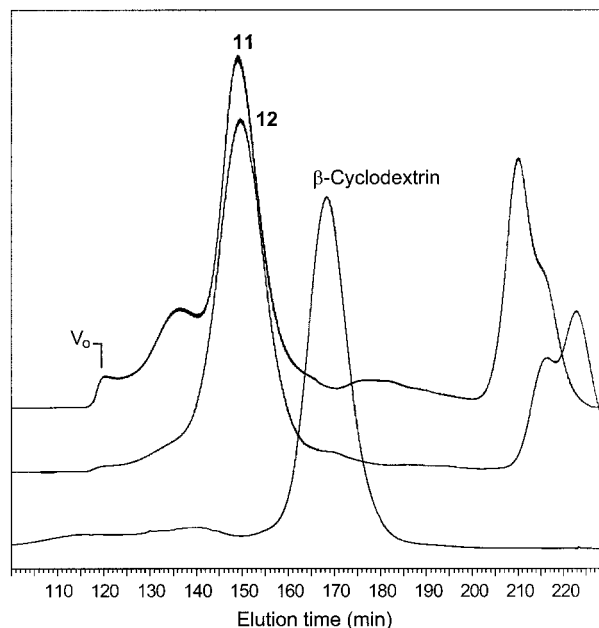
Figure 3. Elution profiles of products from conjugation reactions between TCD 1a and 7 (top), 1b and 7 (middle) obtained on Toyopearl HW-40S column (1.5 \times 85 cm) using a differential refractometer as a detector. Products 11 and 12 were collected between 140 and 160 min. Low molecular weight products were eluted after 200 min, elution time of the void volume was 120 min. For comparison, the elution profile of \beta -cyclodextrin obtained in the same column (peak maximum at 170 min) is shown.
